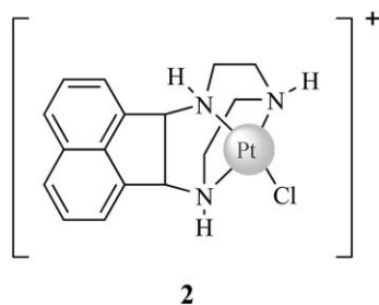
Fig. 2 Pt(II)-intercalative compound 2 . 9
